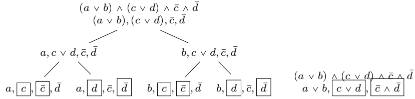
Fig. 9. A redundant tableau and a non-redundant one of the same formula
