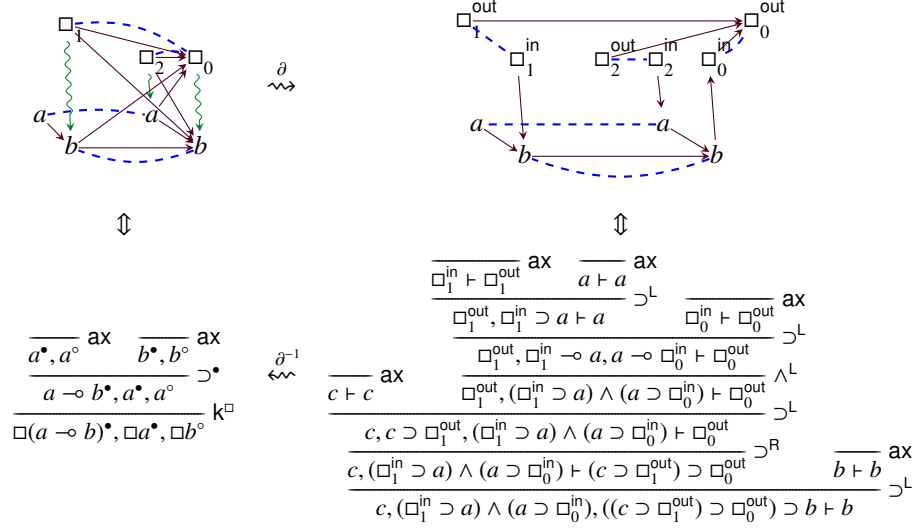
Fig. 9. A K-arena net \mathcal{G} with associated formula \square(a \supset b) \supset (\square a \supset \square b) (the axiom k_1 ), its corresponding arena \partial(\mathcal{G}) , the derivation associated to \mathcal{G} and the derivation associated to \partial(\mathcal{G})
